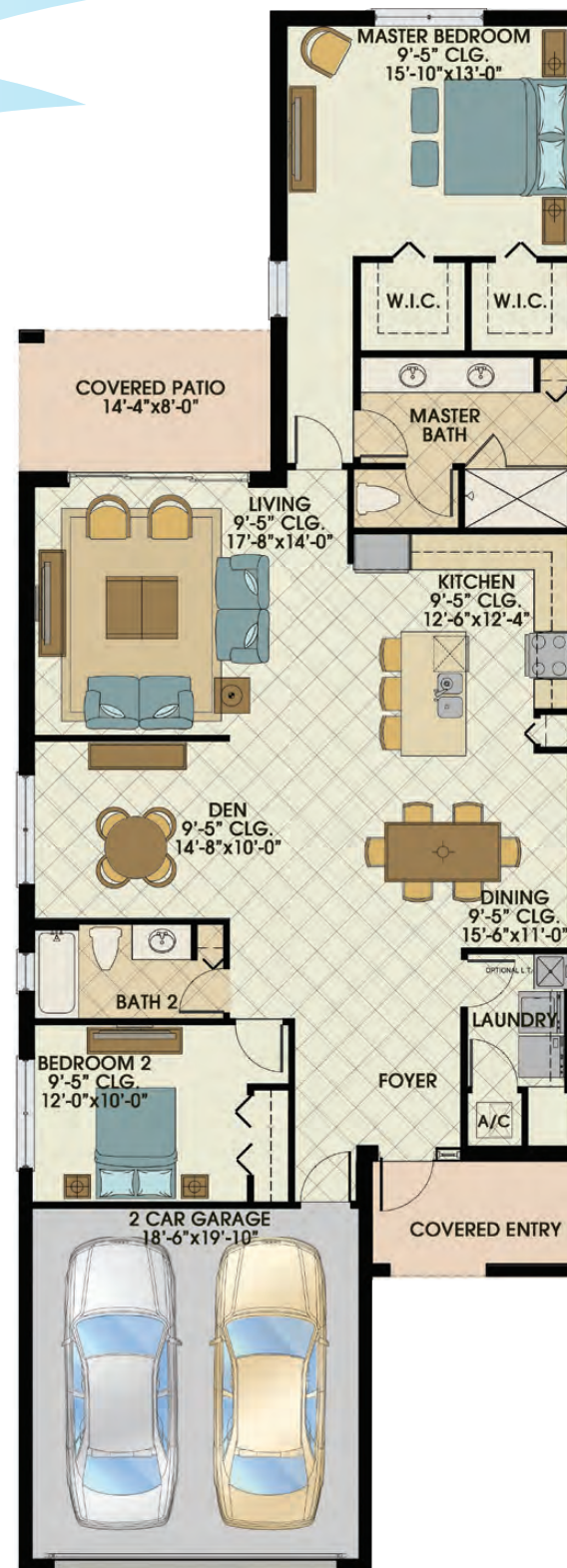
1ST FLOOR PLAN
